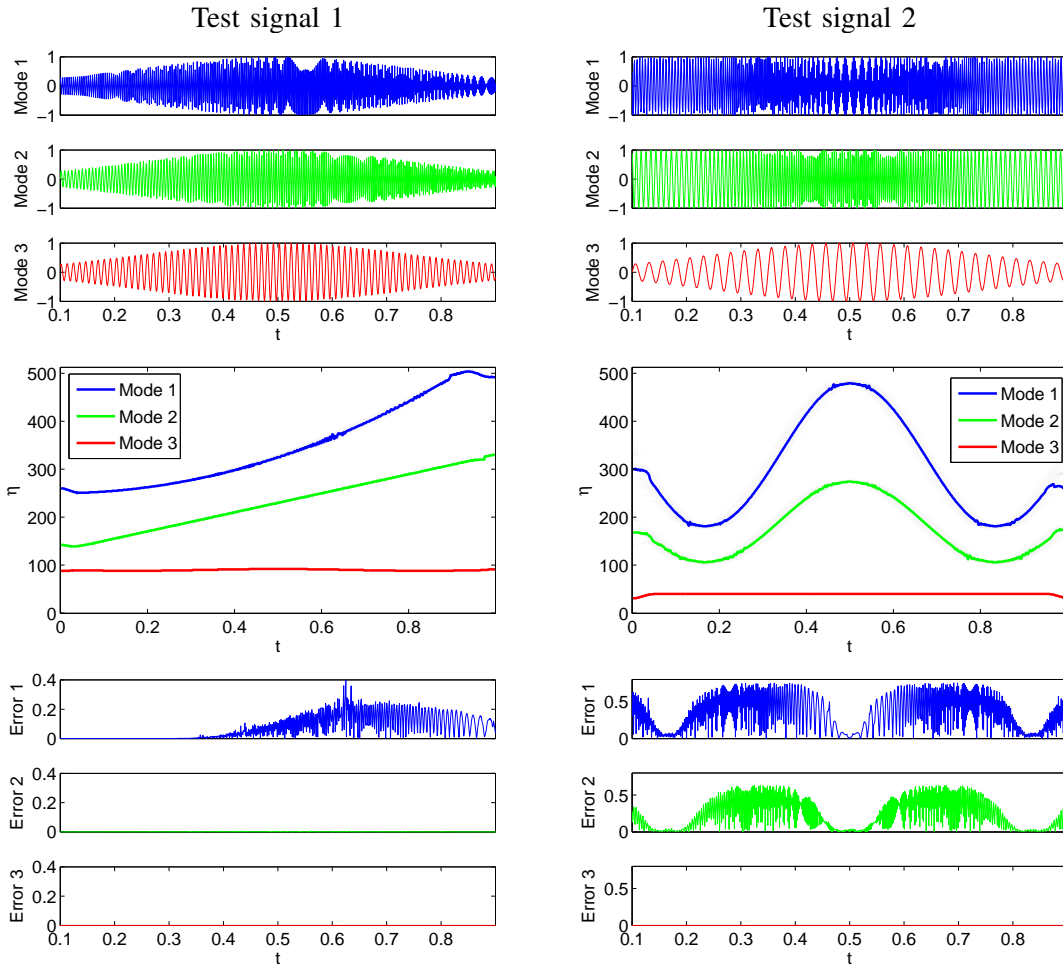
Figure 2. Illustration of mode retrieval based on FSST on test-signals 1 (left) and 2 (right). From top to bottom: the three modes making up the test-signals, their SST with the estimated ridges superimposed, and the reconstruction error. SNR after reconstruction for modes 1, 2 and 3 equals 14, 51 and 70 dB for test-signal 1, and 5, 7 and 70 dB for test-signal 2, respectively. We use d = 5 in the reconstruction (see equation (8)), and \beta = 0 , \lambda = 0.02 for the ridge extraction (see equation (14)).
