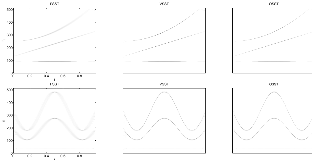
Figure 4. From left to right, magnitude of FSST, VSST and OSST for test-signals 1 (top) and 2 (bottom).
