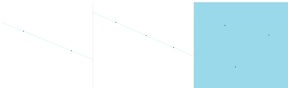
Figure 2: Affine hulls of sets of points
