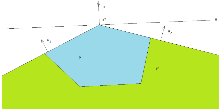
Figure 8: Lemma 3.20: The supporting linear functional u can be represented as a combination of the functionals a_1, a_2 corresponding to the active constraints with nonnegative coefficients.
