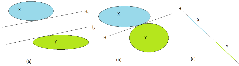
Figure 7: (a) H_1, H_2 separate X, Y strongly; (b) H separates X, Y properly; (c) H does not separate X, Y .
