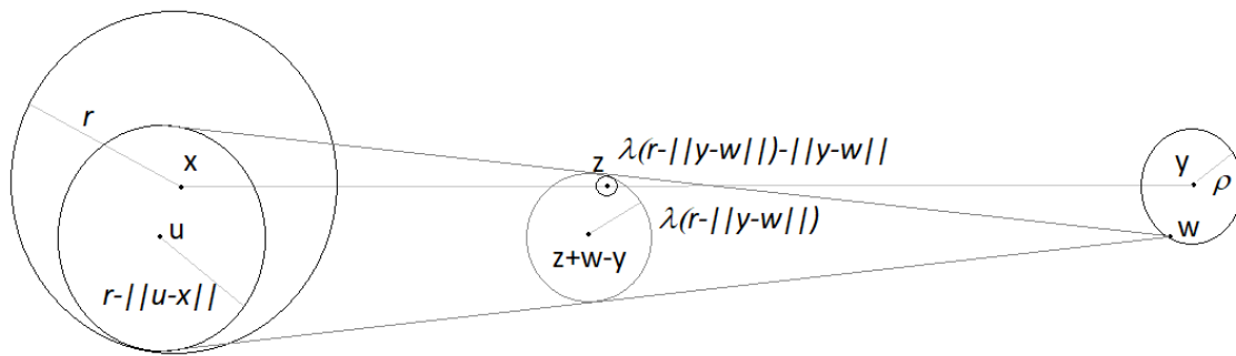
Figure 4: Proof of Lemma 3.8. Radii are shown in italic .
