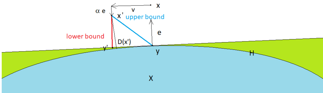
Figure 6: Upper and lower bound on D(x') .
