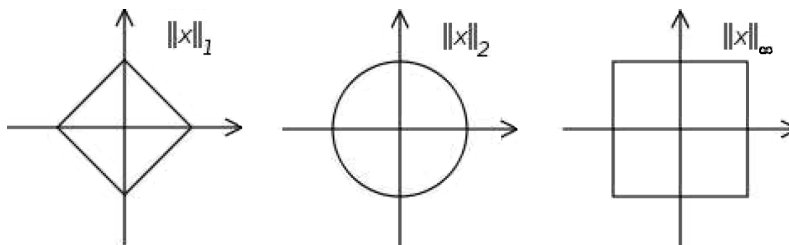
Figure 1: Unit balls of some vector p -norms in the plane
