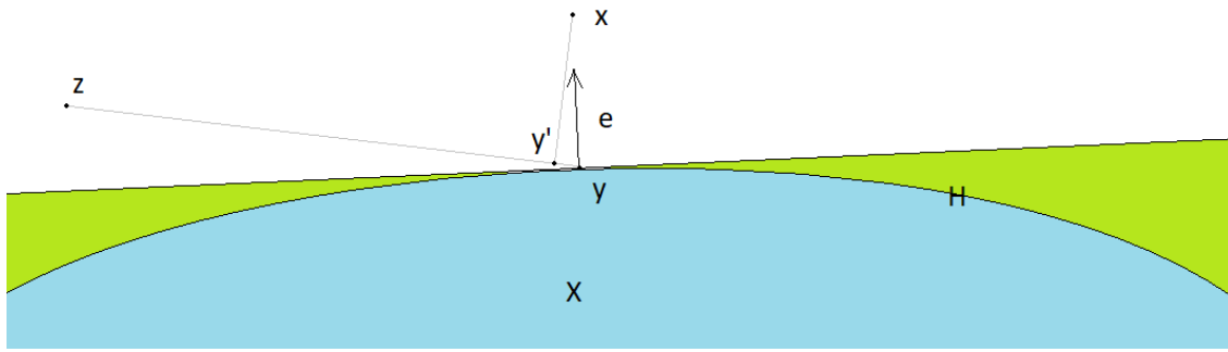
Figure 5: Were z \in X , then y' , which is closer to x than y , would also be in X .
