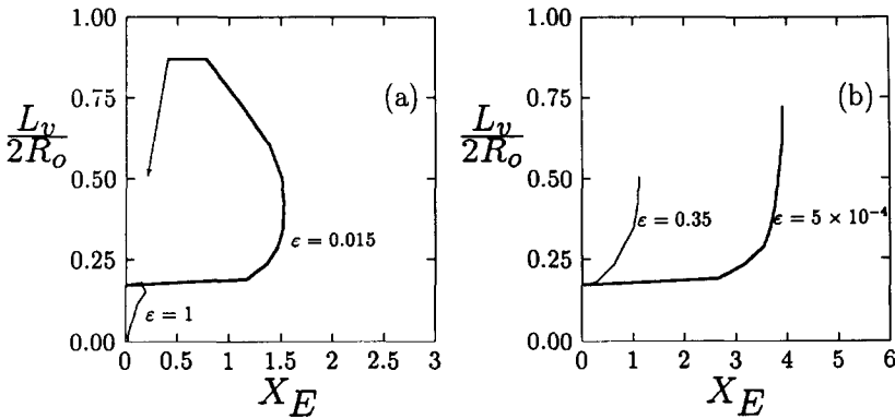
Fig. 12. Reattachment length: (a) exponential version; (b) linear versions
