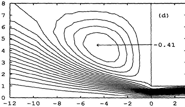
Fig. 9. Linear version ( \epsilon = 5 \times 10^{-4} ): vortex developments: (a) \lambda\dot{\gamma}_w = 2.0 ; (b) \dot{\gamma}_w = 4.6 ; (c) \lambda\dot{\gamma}_w = 14 ; (d) \lambda\dot{\gamma}_w = 69 .
