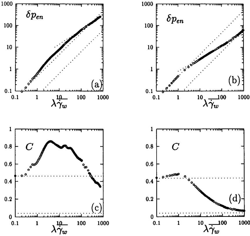
Fig. 13. Exponential version: pressure drop: (a) \epsilon = 0.015 , (b) \epsilon = 1 ; Couette correction: (c) \epsilon = 0.015 , (d) \epsilon = 1 .
