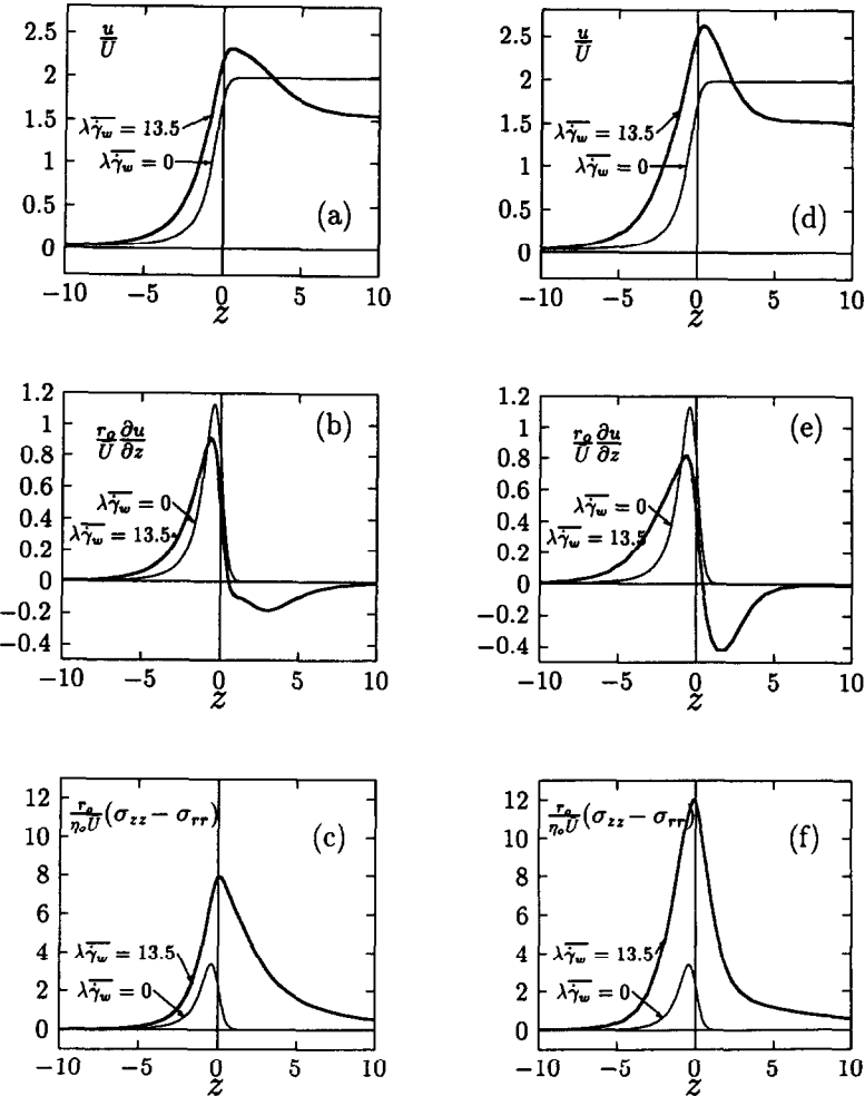
Fig. 16. Profiles along the axis: exponential version \epsilon = 0.015 , \lambda \dot{\gamma}_w = 13.5 : (a) velocity; (b) elongational rate; (c) first normal stress difference; linear version \epsilon = 5 \times 10^{-4} , \lambda \dot{\gamma}_w = 13.5 : (d) velocity; (e) elongational rate; (f) first normal stress difference.
