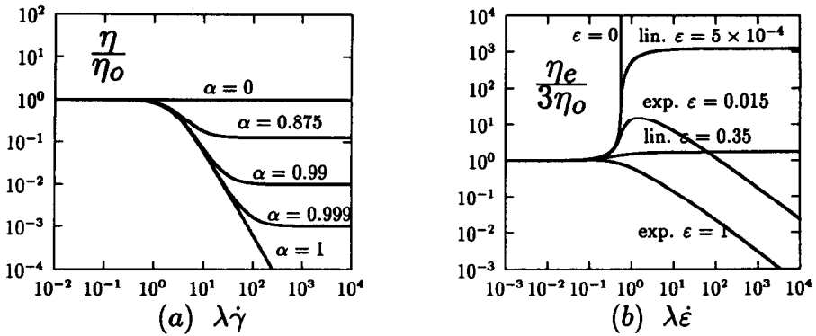
Fig. 1. Simple flows: (a) shear viscosity ( \epsilon = 0.015 , a = 0.9 , exponential version); (b) elongational viscosity ( \alpha = 0.875 , a = 0.9 ).
