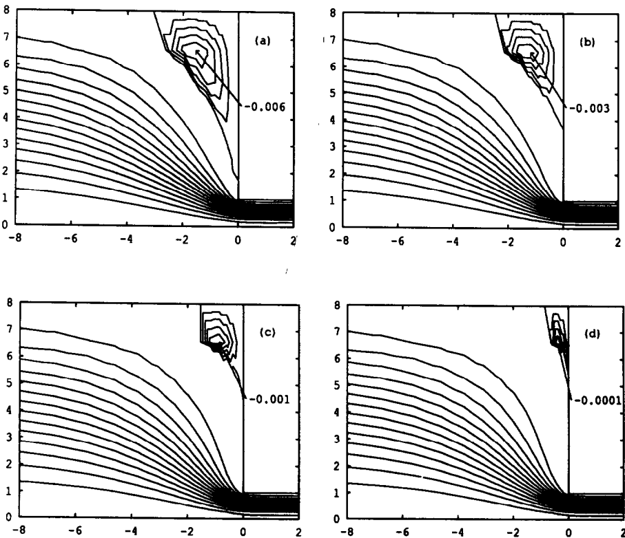
Fig. 8. Exponential version ( \epsilon = 1 ): vortex developments: (a) \overline{\lambda\dot{\gamma}_w} = 4 ; (b) \overline{\lambda\dot{\gamma}_w} = 19 ; (c) \overline{\lambda\dot{\gamma}_w} = 52 ; (d) \overline{\lambda\dot{\gamma}_w} = 182 .
