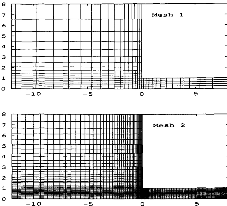
Fig. 6. Partial view of the finite element meshes.
