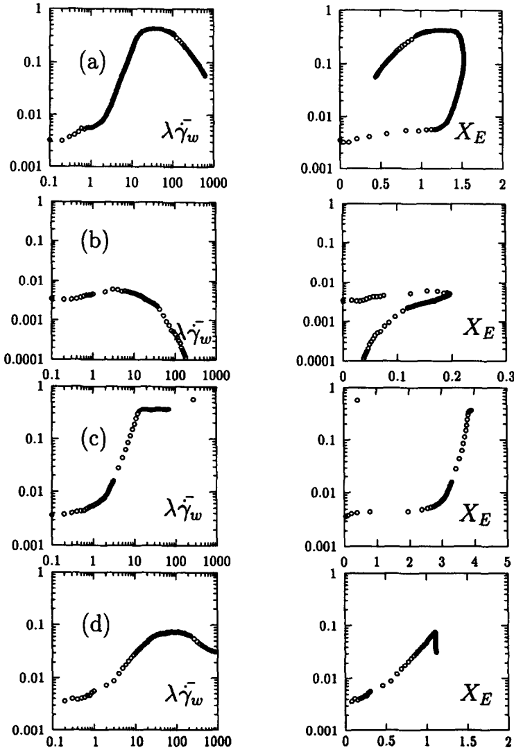
Fig. 11. Vortex activity: exponential version: (a) \epsilon = 0.015 , (b) \epsilon = 1 ; linear version: (c) \epsilon = 5 \times 10^{-4} , (d) \epsilon = 0.35 .
