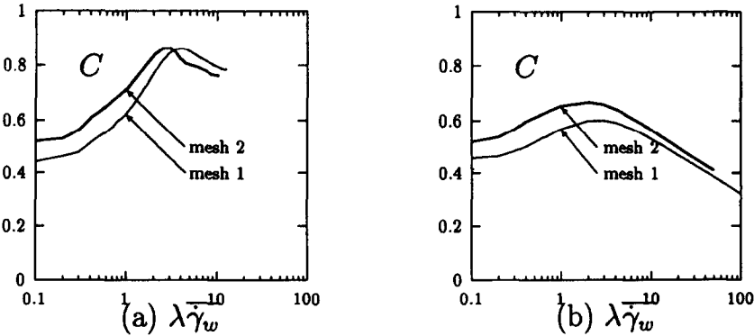
Fig. 15. Mesh sensitivity for the Couette correction: (a) exponential version ( \epsilon = 0.015 ); (b) linear version ( \epsilon = 0.35 ).
