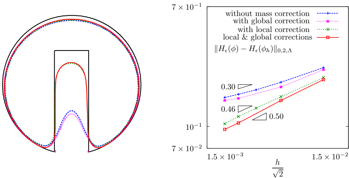
FIG. 1. The Zalesak disk: (a) initial position (black and dotted) and after one rotation: without correction (blue and dotted line), with global correction (magenta and dashed), with local correction (green and dashed), with local and global corrections (red and solid line) ; (b) convergence properties in log-log scale.
