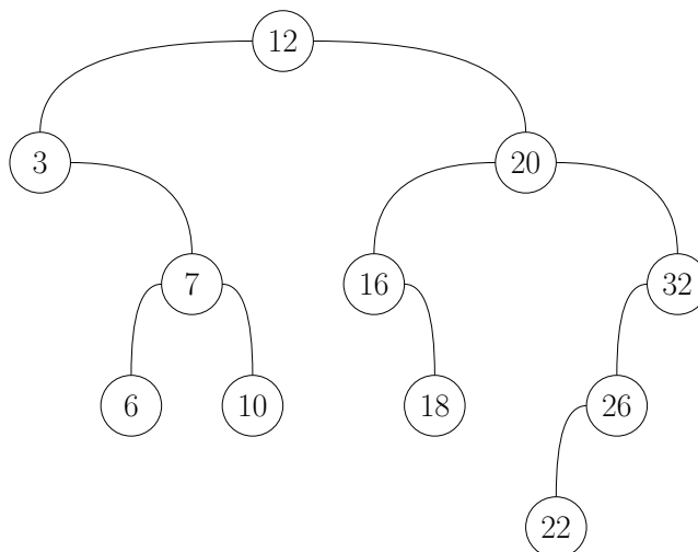
FIGURE 10.4 – Un ABR pour l'ensemble {3, 6, 7, 10, 12, 16, 18, 20, 22, 26, 32}.
