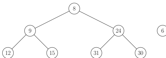
FIGURE 12.14 – On extrait 6.
