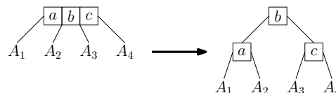
FIGURE 11.28 – Racine.
