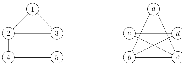
FIGURE 14.12 – Deux graphes isomorphes.
