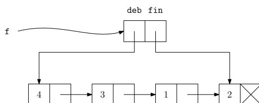
FIGURE 7.12 – La file \leftarrow (4, 3, 1, 2) \leftarrow .
