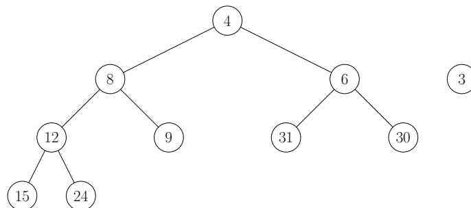
FIGURE 12.12 – On extrait 3.
