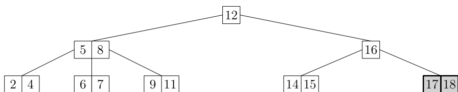
FIGURE 11.15 – Insertion de 17.
