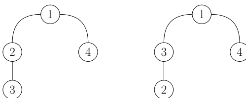
FIGURE 14.31 – Deux arbres distincts : E = \{\{1, 2\}, \{1, 4\}, \{2, 3\}\} et E = \{\{1, 3\}, \{1, 4\}, \{2, 3\}\} .
