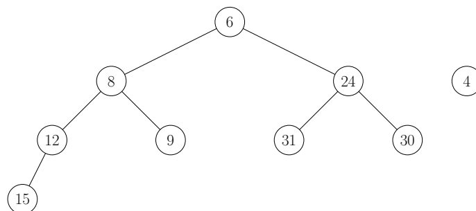
FIGURE 12.13 – On extrait 4.
