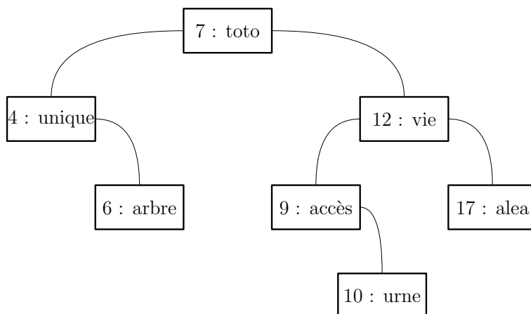
FIGURE 11.12 – Exemple de (int, string) dict.
