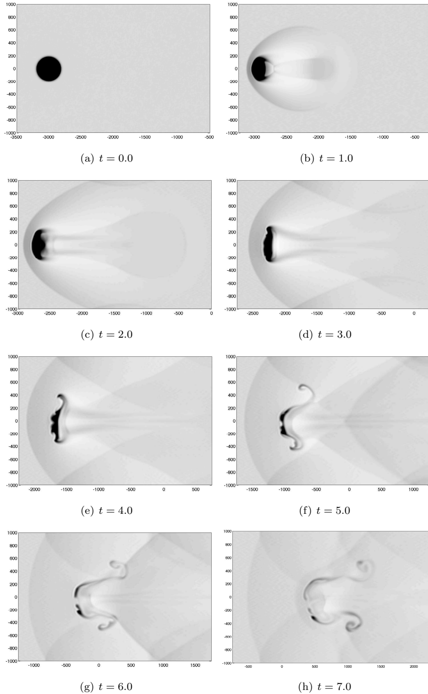
Fig. 1. Astrophysics test-case: density in the symmetry plane; color range: white \rho = 0 , black \rho = 2e^{-7} M_{\odot} \text{kpc}^{-3} ; free-stream coming from the left
