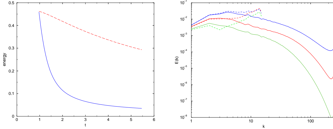
FIGURE 4. Energy decay (left picture) and energy spectrum at times t = 1.28, 2.45 and 5.46 (right picture) for filtered reference DNS (energy carried by the first 32 modes) (solid) and a DNS with N = 32 modes (dashed)
