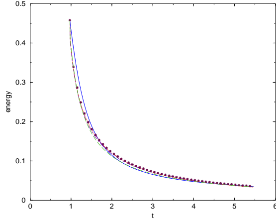
FIGURE 6. Energy decay: solid line: reference DNS filtered on 32^3 modes; dashed line: Smagorinsky model with C_S = 0.27 ; dot-dashed line: selective Smagorinsky model, with \beta_0 = 15^0 and C_S = 0.36 ; stars: selective Smagorinsky model, with \beta_0 = 5^0 and C_S = 0.29 ; dotted line: selective anisotropic model with C_a = 0.4
