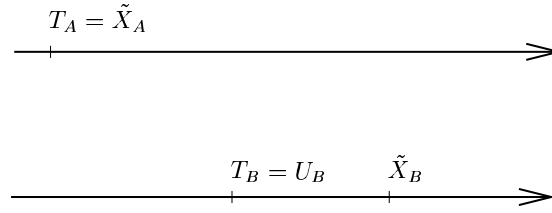
Figure 2.4: Case T_A < T_B , \delta_A = 1 , \delta_B = 0 .
