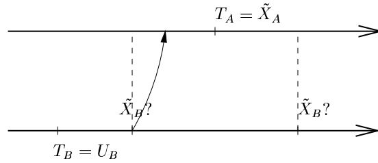
Figure 2.5: Case T_B < T_A , \delta_A = 1 , \delta_B = 0 .
