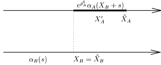
Figure 2.2: Case X_B < X_A : \tilde{X}_A = X_B + X'_A
