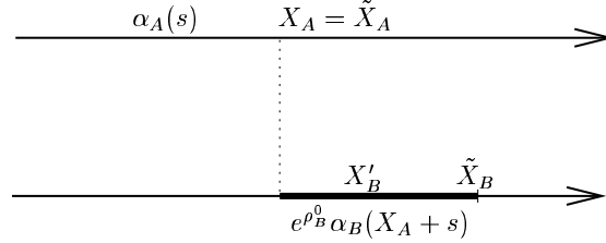
Figure 2.1: Case X_A < X_B : \tilde{X}_B = X_A + X'_B
