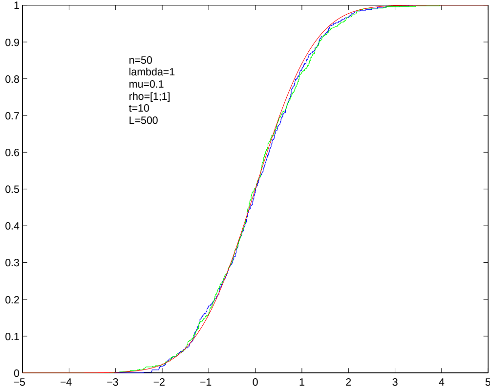
Figure 2.6: Empirical distribution functions of the estimators in comparison with the standard Gaussian distribution function
